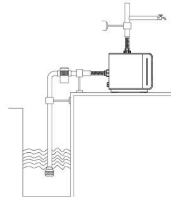
Fig. 4 Suction from well or tank
