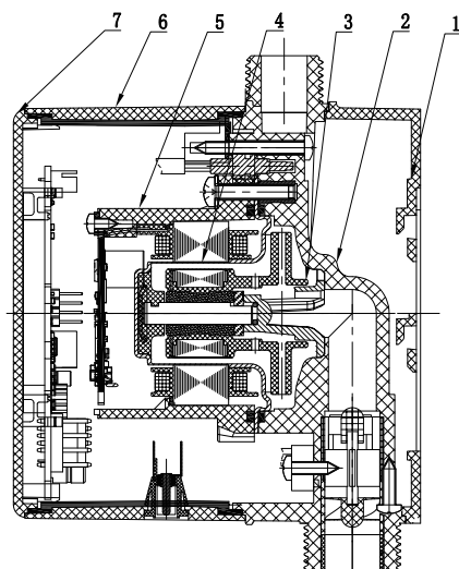
Fig. 7 Sectional drawing
