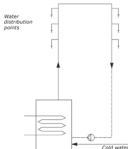
Fig. 11 Functional drawing of one-circuit hot water recirculation
