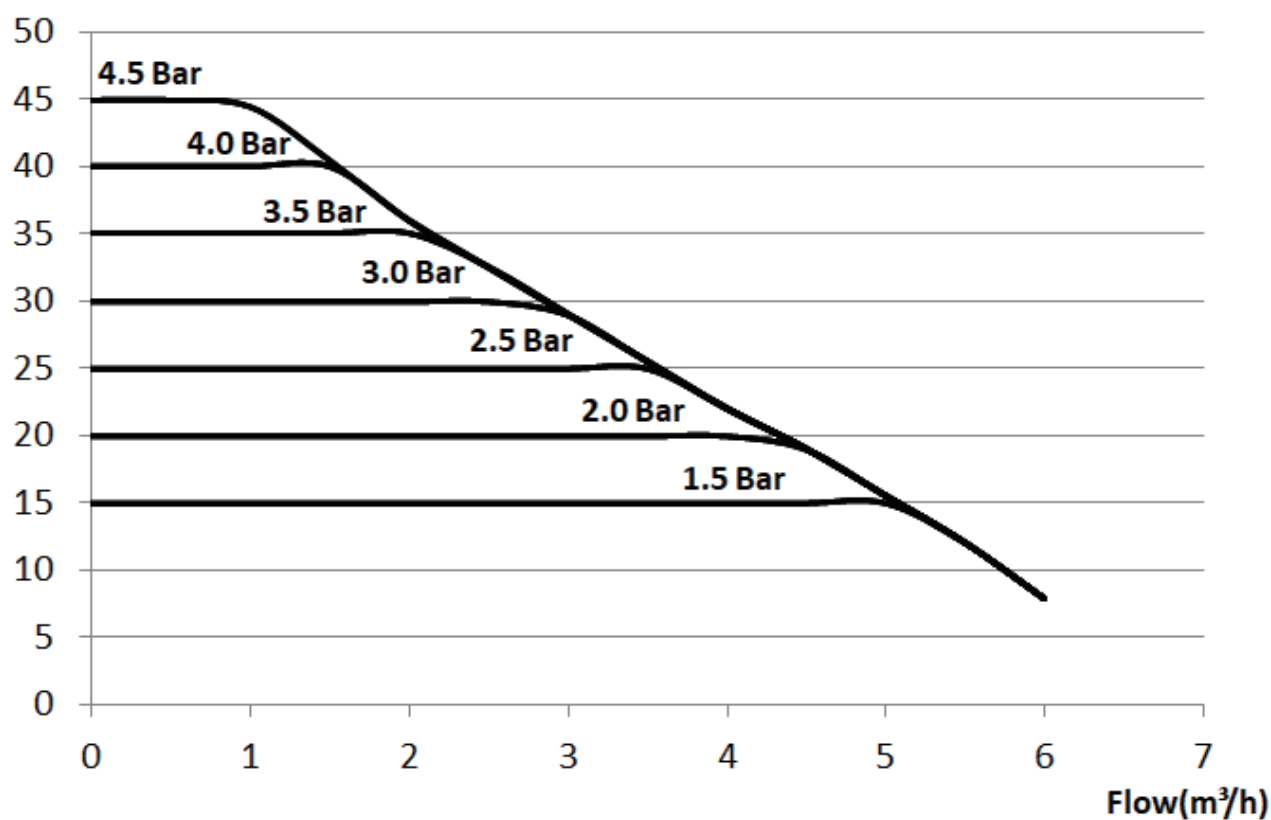
Fig.6 Performance curves
