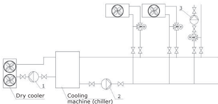
Fig. 32 Functional drawing of air conditioning system
