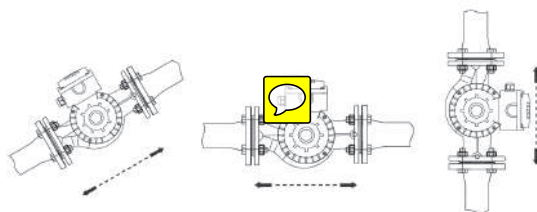
Fig. 53 Installation options
