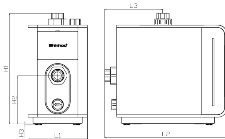
Fig.7 External dimensions
