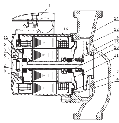
Fig. 7 Sectional drawing
