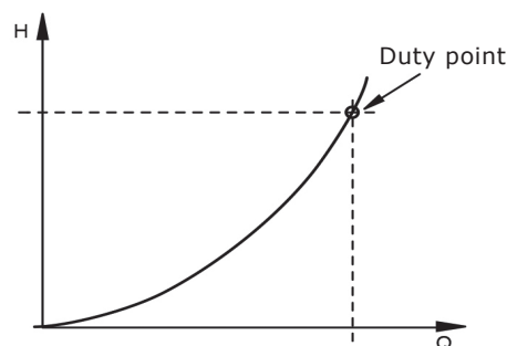
Fig. 1 System characteristic
