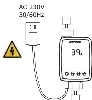
Fig.6 Wiring Diagram
