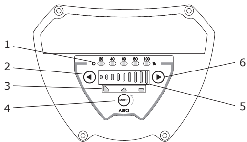
Fig. 41 Operating panel
