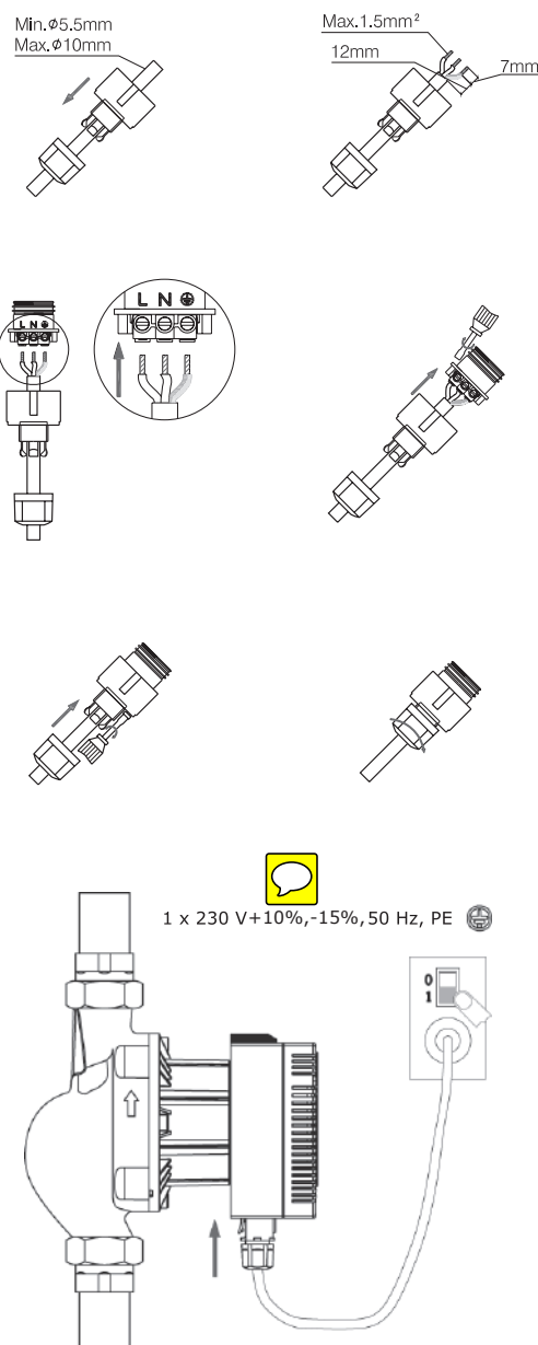
Fig. 36 Electrical connection
