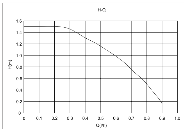
Fig.4 Performance curve
