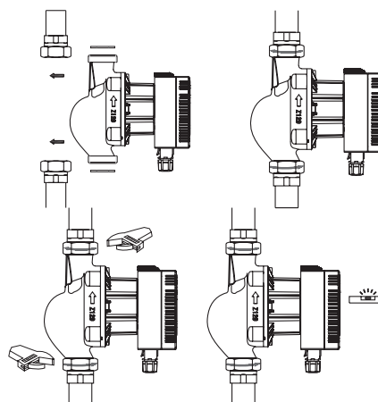
Fig. 35 Pump installation
