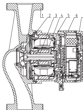
Fig. 6 Sectional drawing
