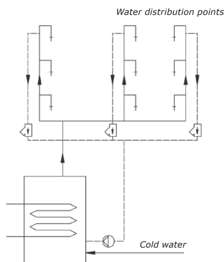
Fig. 12 Functional drawing of multi-circuit hot water recirculation
