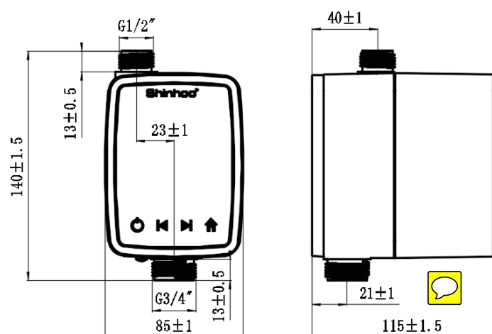
Fig.8 Installation dimension
